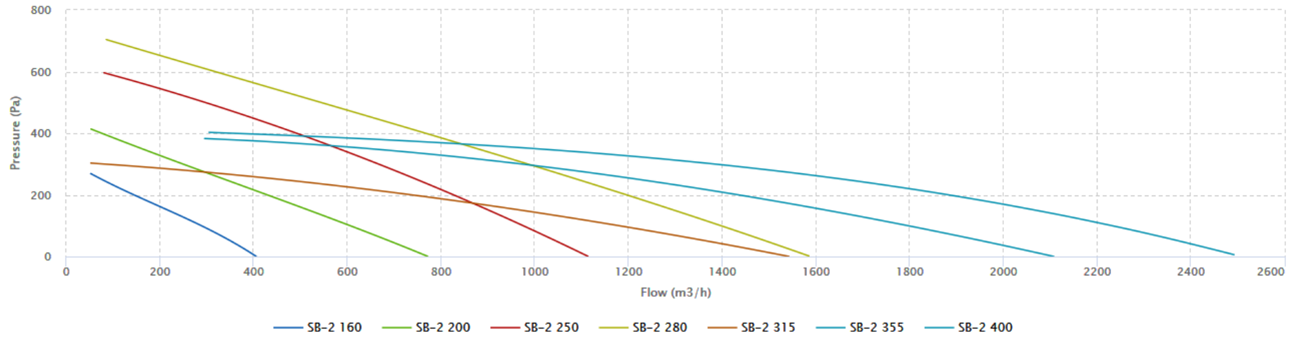
Flow-Pressure
